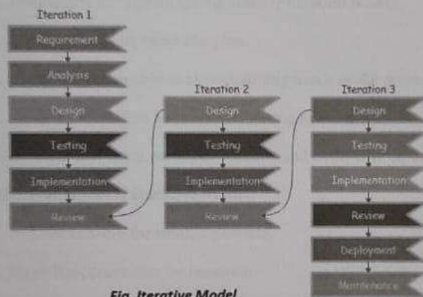
Fig. Iterative Model
